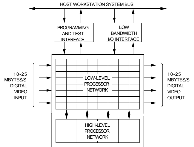
Figure 2: The data-flow computer architecture
