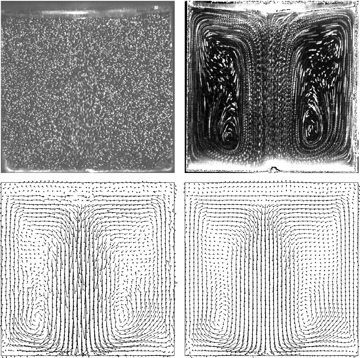
Fig. 6. Real particle sequence (four 496 \times 496 images). Water freezing in a lid cooled cubical cavity. Top left: particle image; top right: 15 superimposed similar images; bottom left and right: recovered velocity fields from two images and four images. Velocity fields are displayed using a non linear scale. The average module of the extracted velocity field is of 4.4 pixels/frame with a maximum of 27.4 pixels/frame.
