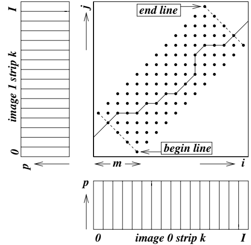
Fig. 3. Image slicing
