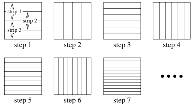
Fig. 4. Image slicing
