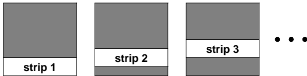
Fig. 1. Image slicing
