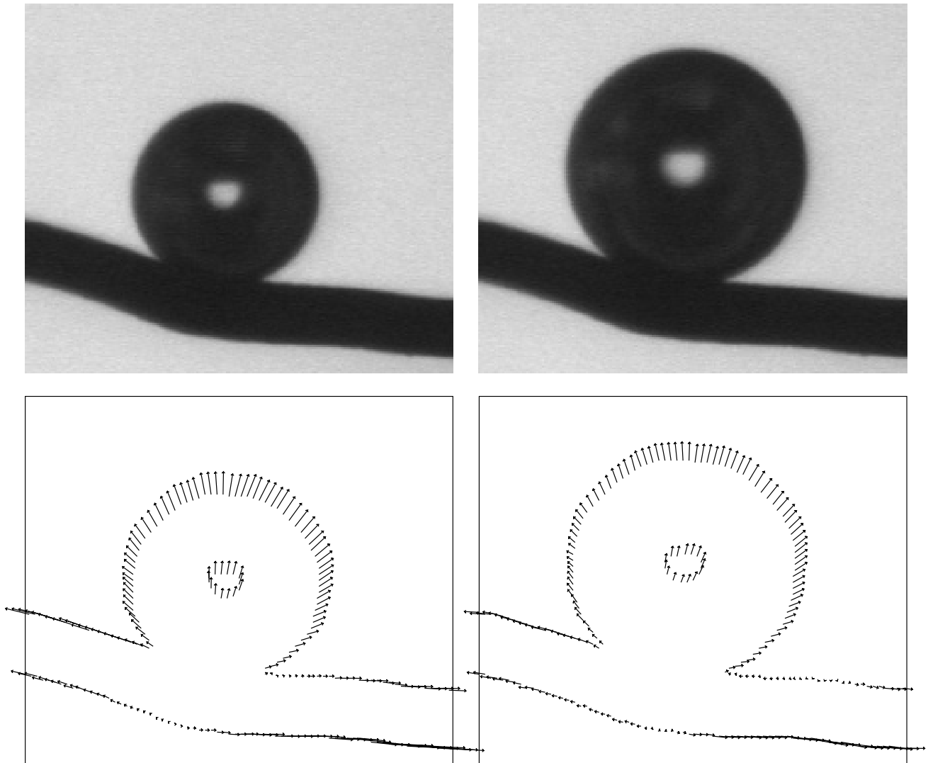
Fig. 8. Bubble sequence (nine 215 \times 185 images). Microscopic images of a vapor bubble growing on a thin heated wire. Methyl alcohol, images taken every 40ms, illumination time 100ns, mean bubble diameter 180 \mu m. Top left and right: first and last image of the sequence, bottom left and right: velocities obtained from the first four and the last four images of the sequence. Velocity fields are computed on the whole image but displayed only on contours. Vectors represent the displacement between the first and last image used for the computation (absolute scale).
