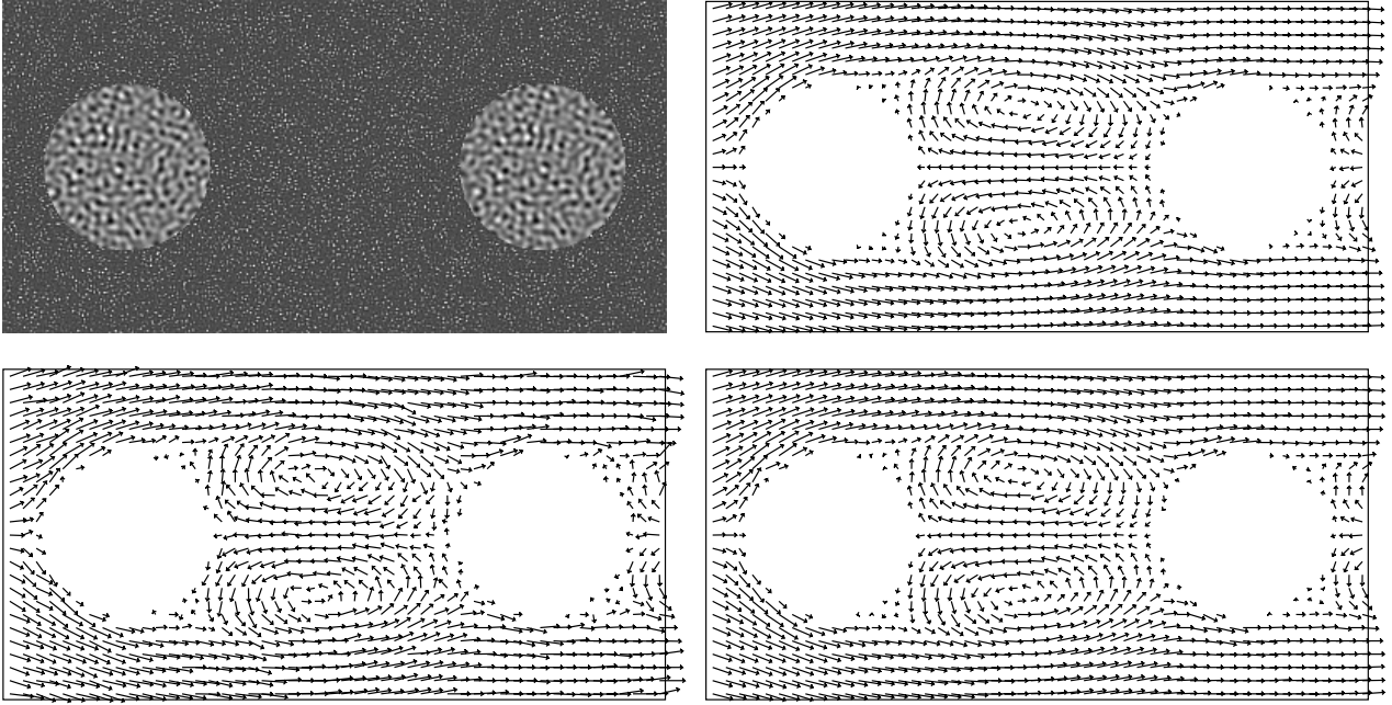
Fig. 5. Synthetic particle sequence (four 800 \times 400 images). Top left: synthetic particle image; top right: original reference velocity field (subsampling 16 times horizontally and vertically), average velocity module is 7.58 pixel/frame; bottom left and right: recovered velocity fields from two images and four images under worst case conditions (20% of additive noise and 20% of particles added or removed). Velocity fields are displayed using a non linear scale.
