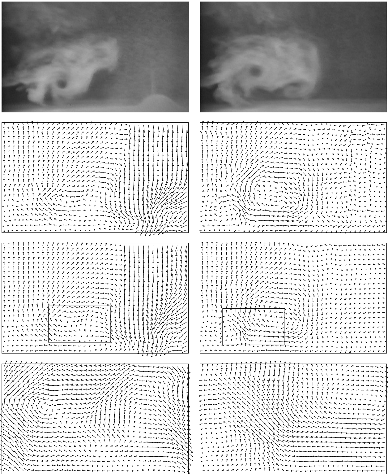
Fig. 7. Smoke sequences (four 700 \times 416 images, extracted from a longer sequence taken by Y. Levy, Technion, Israel). Top row: images from the original sequence; middle top row: velocity fields from 2 images (subsamped 18 times horizontally and vertically); middle bottom row: velocity fields from 4 images (subsamped 18 times); bottom row: 3x zoom of a portion of the velocity fields (subsamped 6 times). Velocity fields are displayed using a non linear scale.
